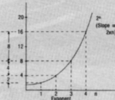
Fig. 3: Exponential Scale.
