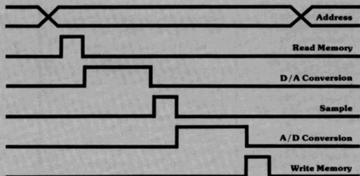
Figure 3: Timing diagram.
