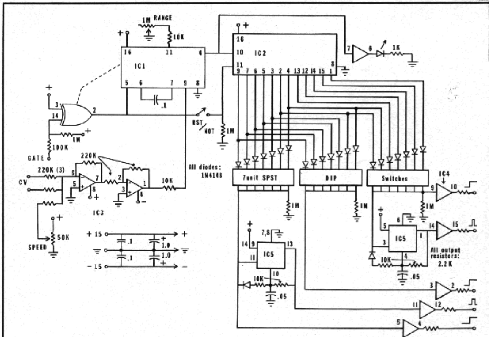
Above, voltage controlled clock schematic. Below, a sampling of event arranger settings and output patterns.
